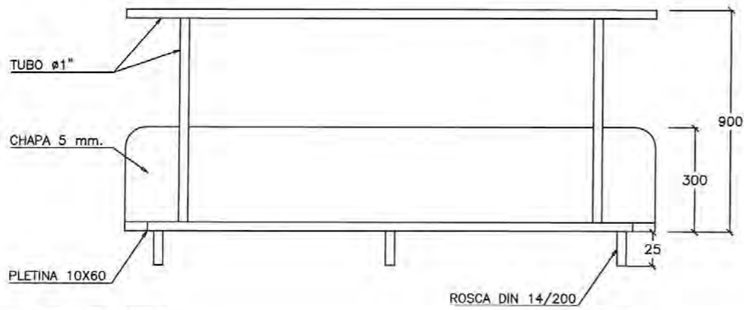
BARANDA
