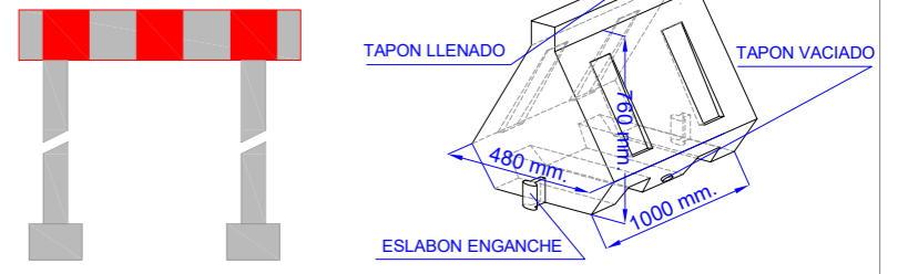
BARRERA NEW JERSEY
